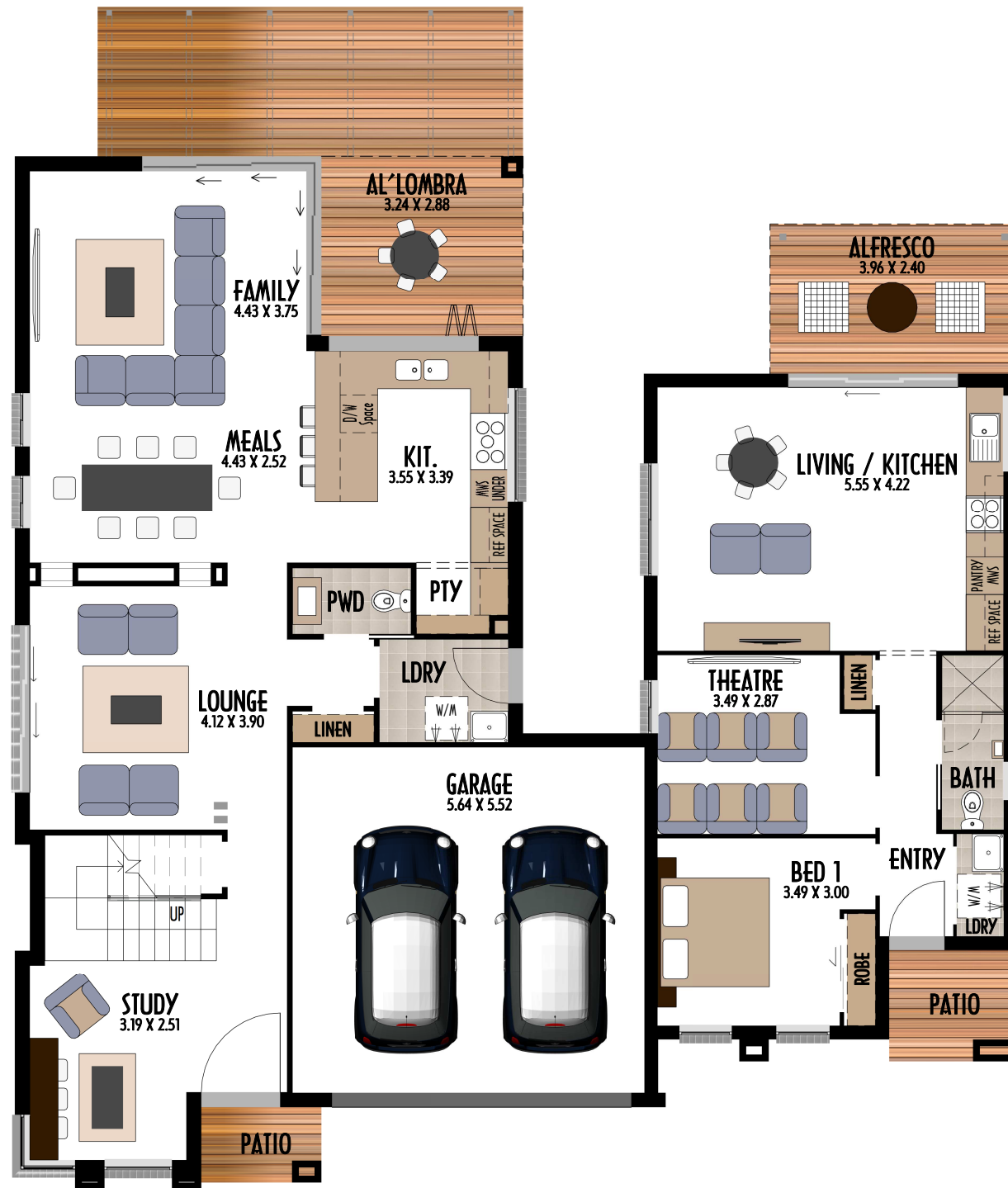
GROUND FLOOR
