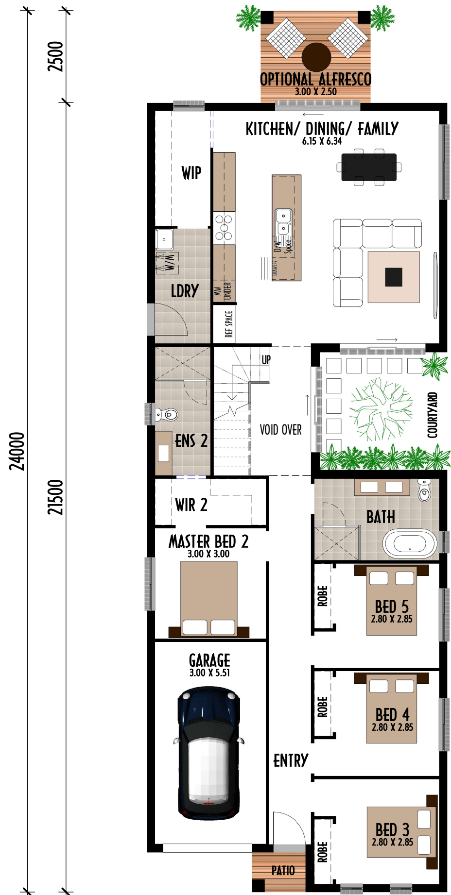
GROUND FLOOR
