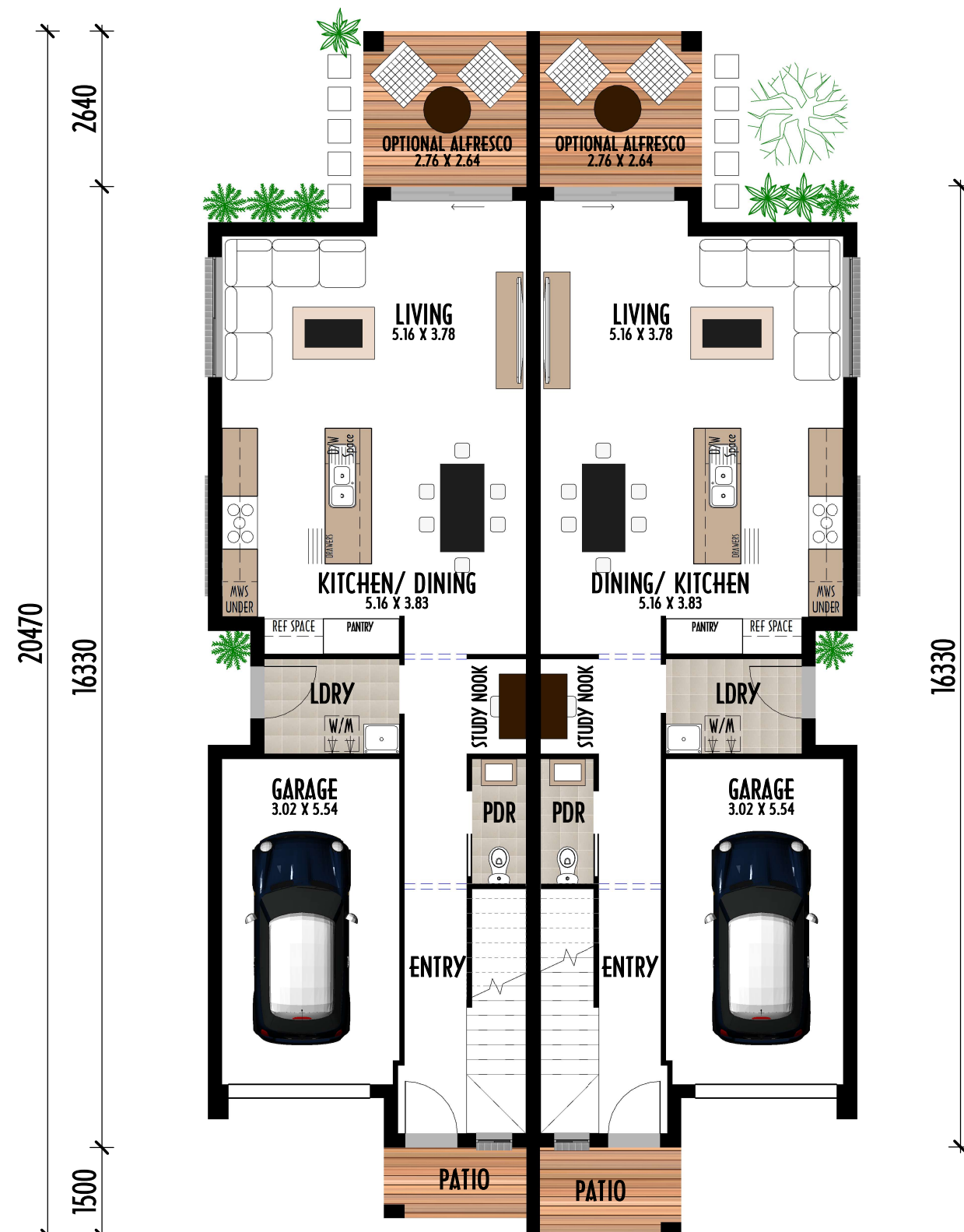
GROUND FLOOR
