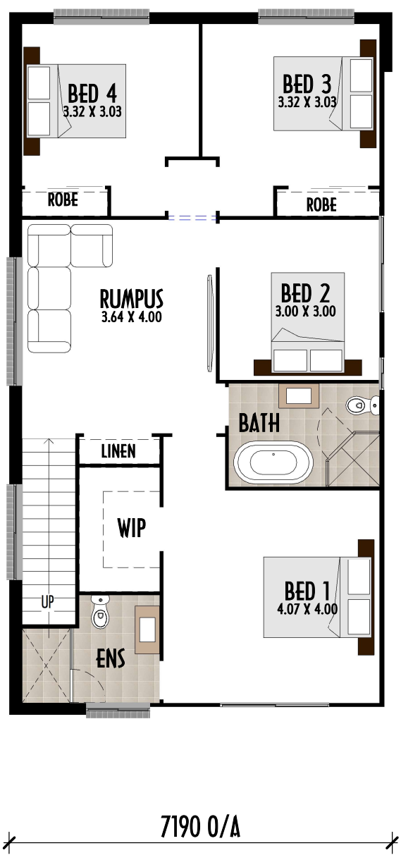
FIRST FLOOR
