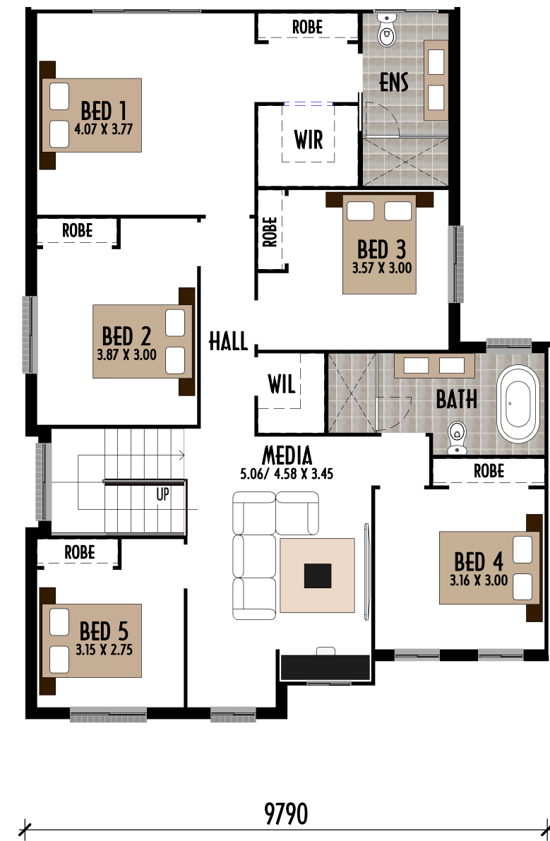
FIRST FLOOR
