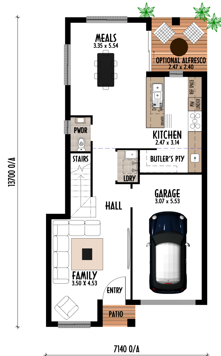
GROUND FLOOR
