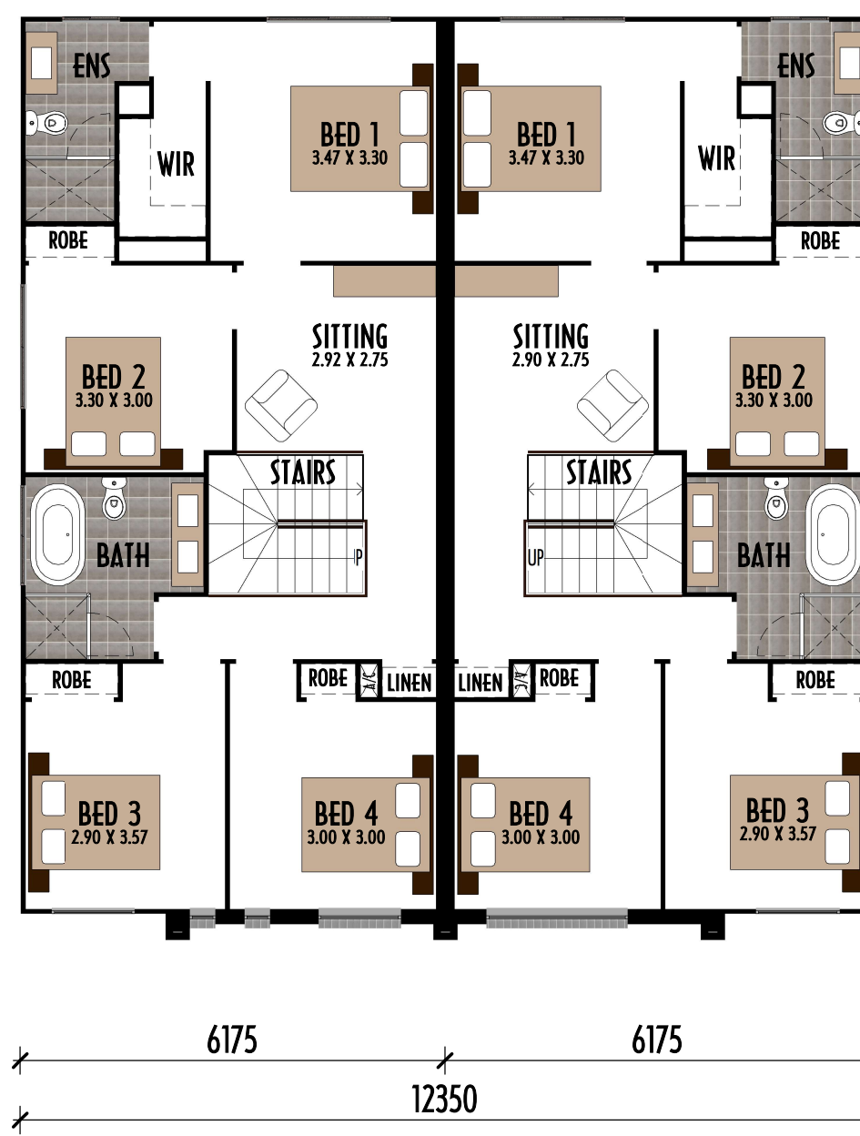
First Floor
