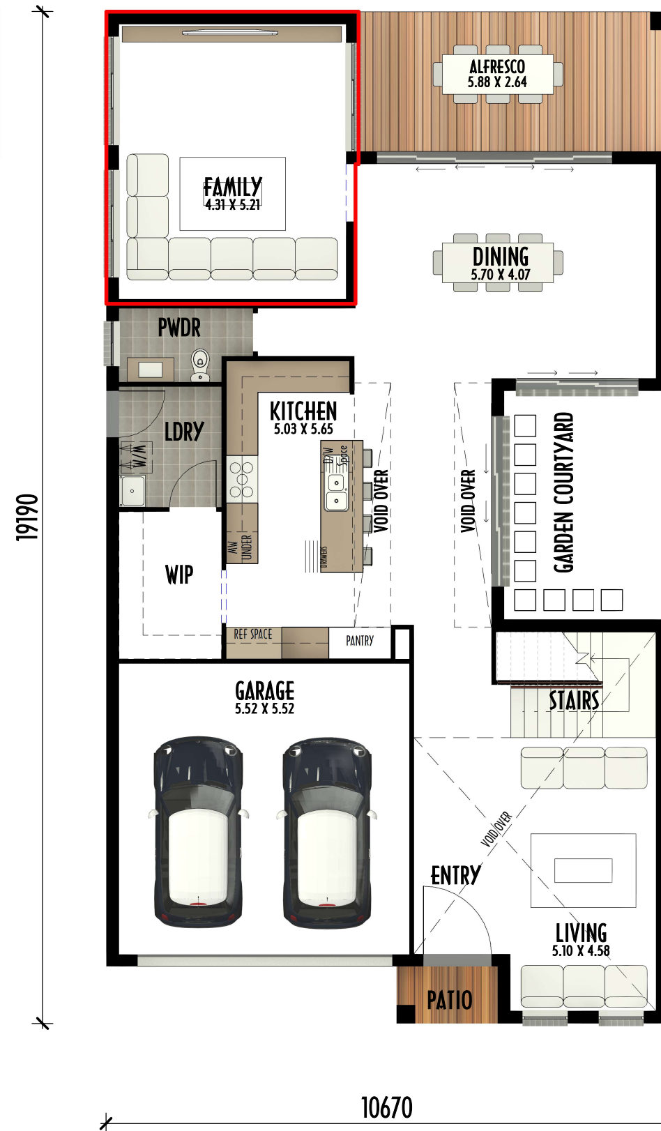
GROUND FLOOR
