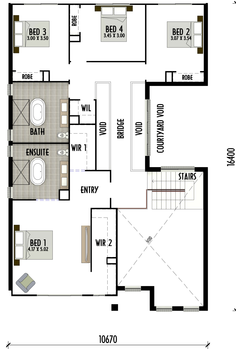
FIRST FLOOR
