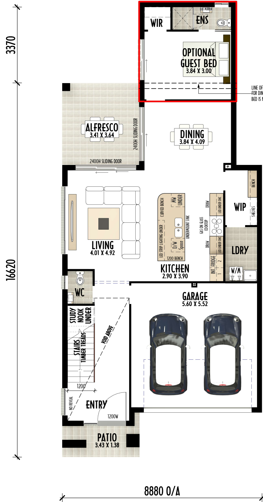
GROUND FLOOR
