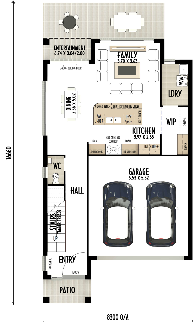
GROUND FLOOR
